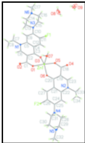
Fig. 1. The asymmetric unit of the title compound showing the showing 50% displacement ellipsoids for non-H atoms.
